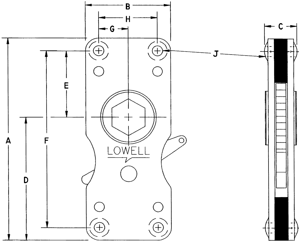
SERIES 700 BODY DIMENSIONS (in inches)
