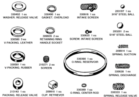
BU0953B Hydraulic pump
