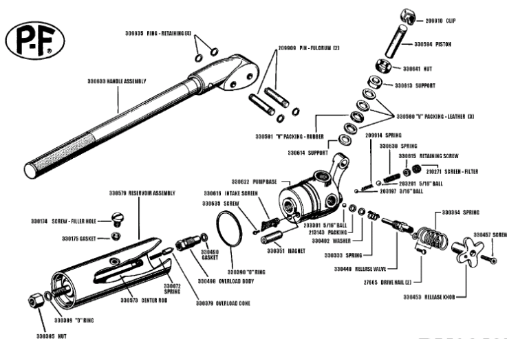
BU0953B Hydraulic pump
